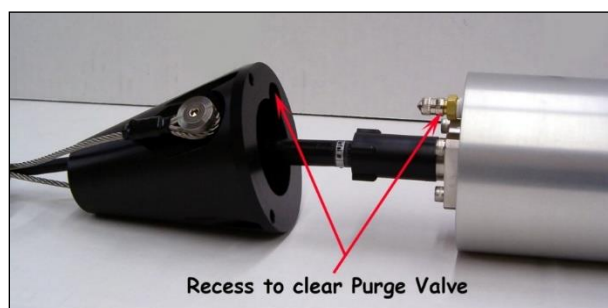
FIGURE 5: ATTACHING THE DROP CONE ASSEMBLY
