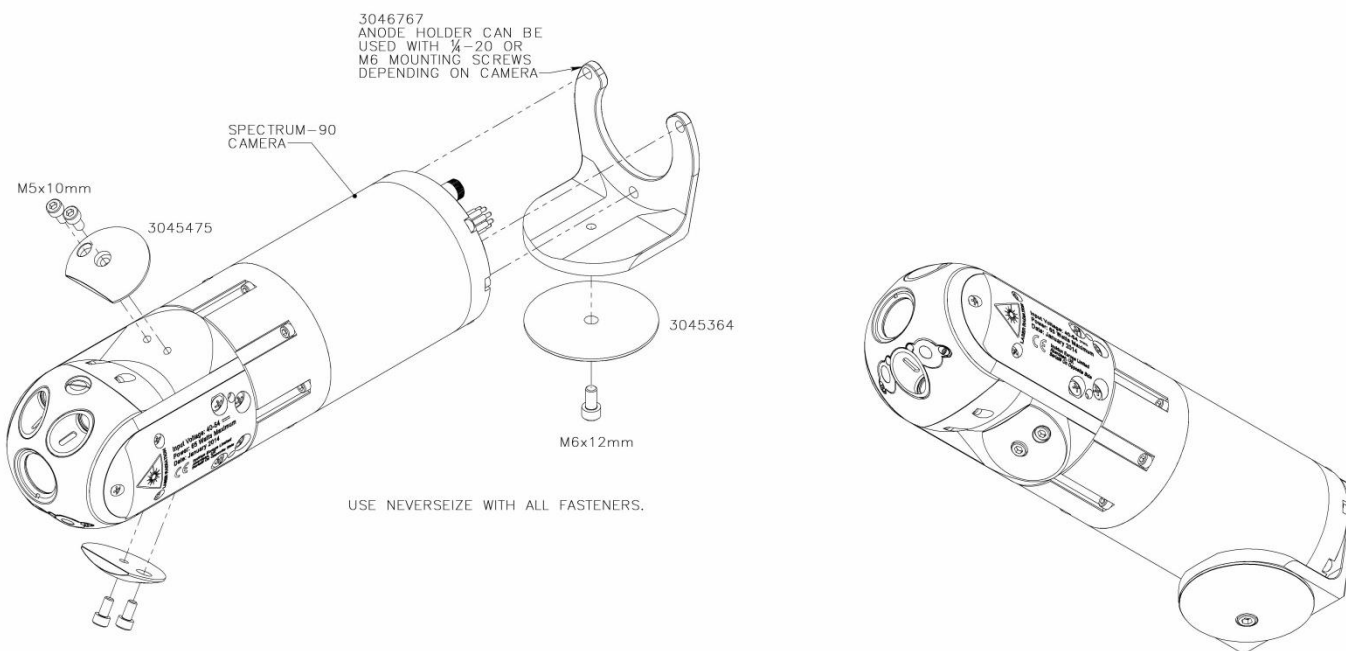
FIGURE 4: ANODE ATTACHMENT
