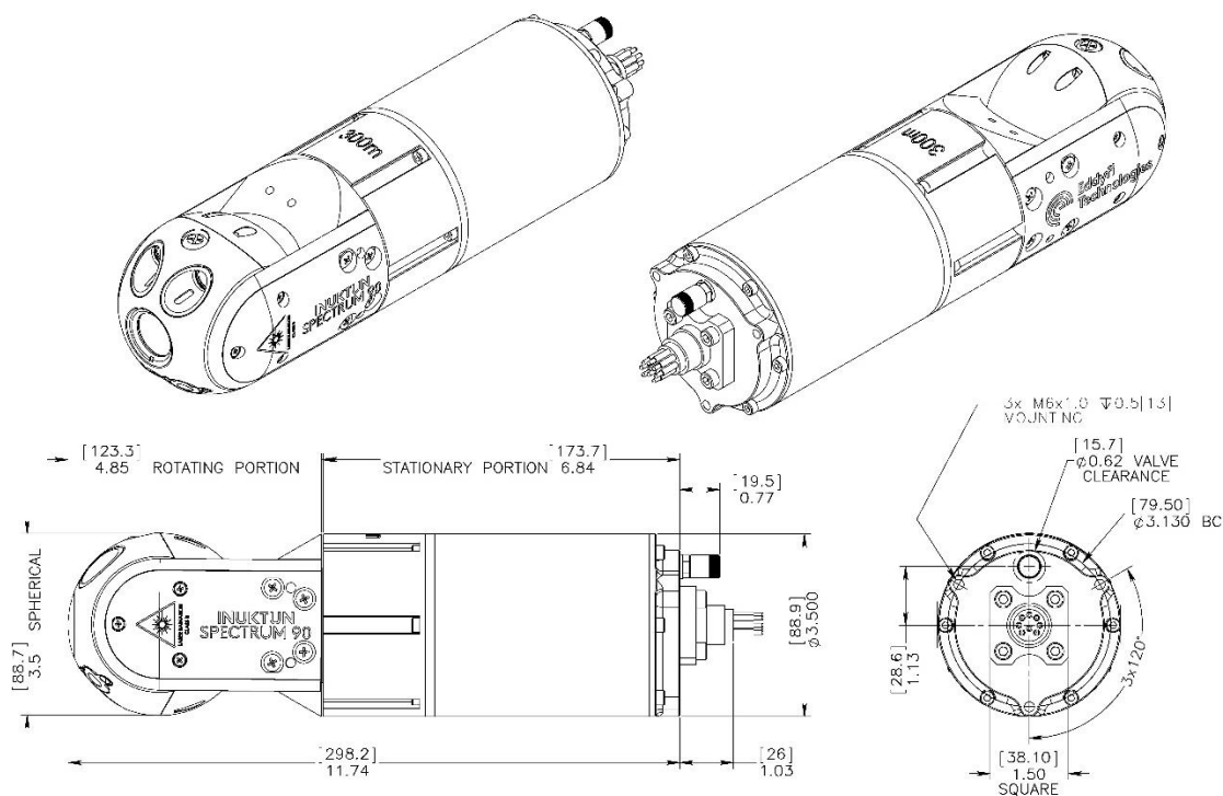
FIGURE 3: SPECTRUM 90™ DEEP WATER CAMERA MOUNTING DIMENSIONS
