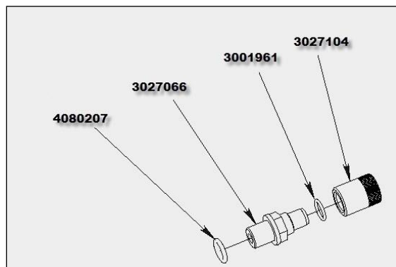
FIGURE 7: DEPTH RATED SCHRADER VALVE ASSEMBLY
