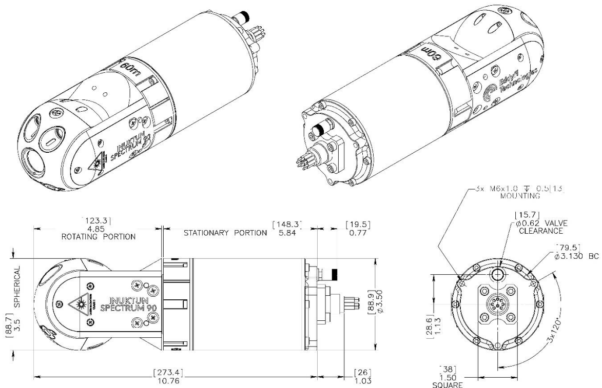
FIGURE 2: SPECTRUM 90™ STANDARD CAMERA MOUNTING DIMENSIONS
