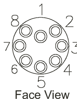
FIGURE 1: SD CONNECTOR PIN-OUT
