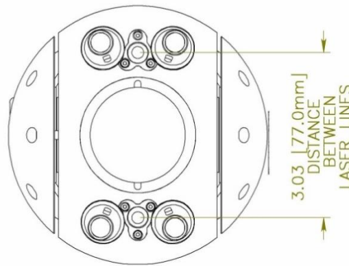
FIGURE 3: LASER LINE SEPERATION DISTANCE
