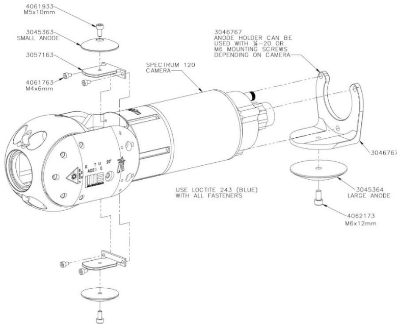
FIGURE 6: GALVANIC CORROSION CONTROL
