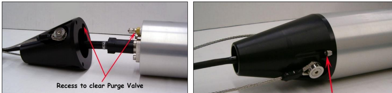
FIGURE 7: ATTACHING THE DROP CONE ASSEMBLY
