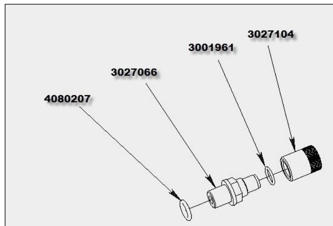
FIGURE 9: DEPTH RATED SCHRADER VALVE ASSEMBLY
