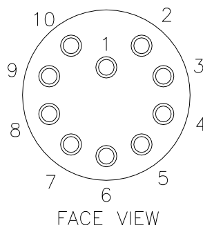
FIGURE 2: HD CONNECTOR PIN-OUT
